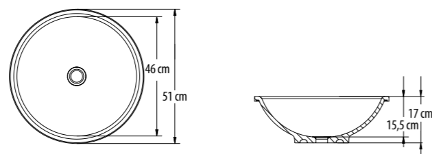
mod. VBS ø 51 cm
