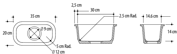
mod. BS 1206 35 x 20 x 14 cm
